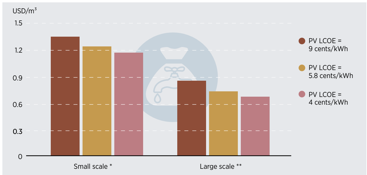
Figure A.4 Levelised water production costs for grid-connected solar PV systems under various LCOE assumptions (USD/m 3 )
