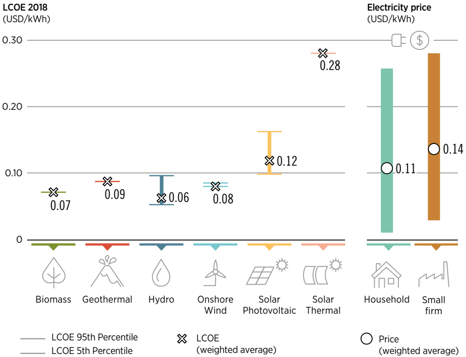
LCOE based on IRENA (2019a) and electricity prices based on Global Petrol Prices (2019). Note: The LCOE data is for projects commissioned in 2018. Real weighted average cost of capital (WACC) is 7.5% for OECD countries and China and 10% for the rest of the world.
