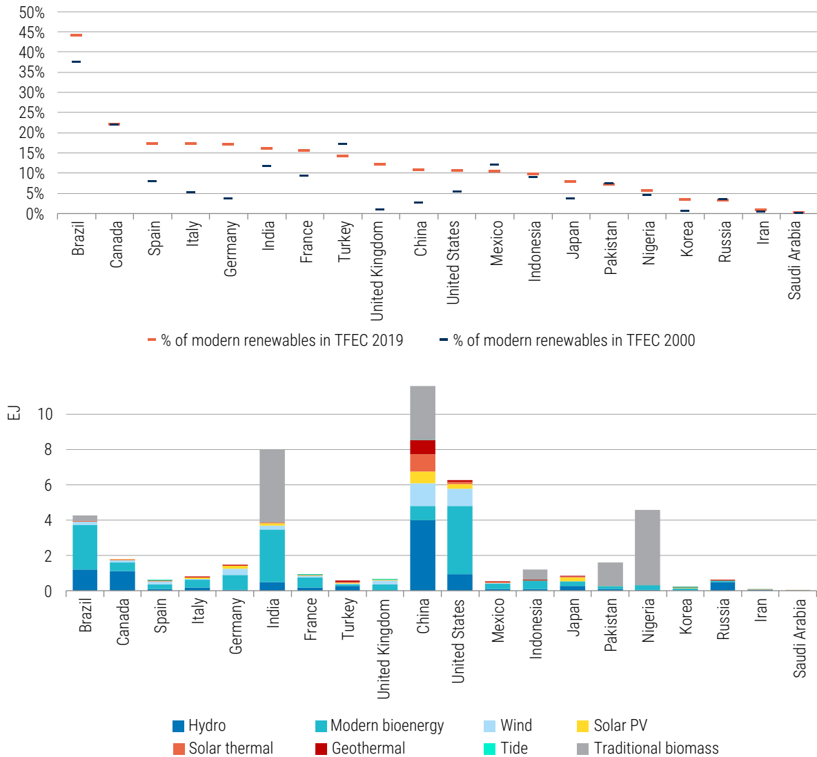
Figure 3.7 • Share of renewables in total final energy consumption, 2000 and 2019, and renewable energy consumption, by source, in the top 20 energy-consuming countries, 2019
